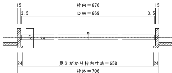
■横断面図[間口3尺]
