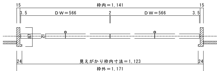
■横断面図[間口4.5尺]
